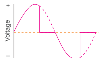
Trailing-edge dimmer
