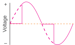
Leading-edge dimmer
