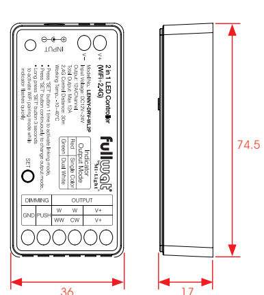
LENNY-DRV-WL2P
