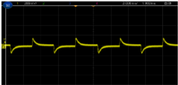
Figure 5. 50% - 75% load dynamic
