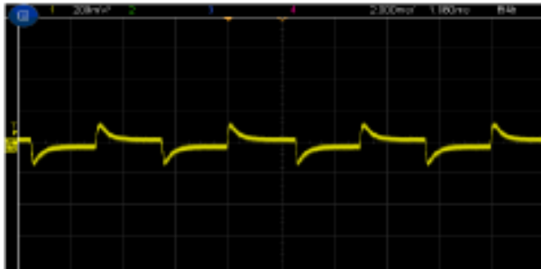
Figure 4. 25% - 50% load dynamic
