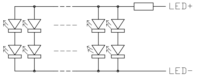
Backlight Circuit (No. of LEDs = 28pcs) Scale=free
